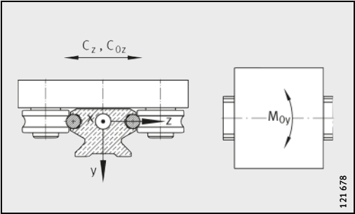
Load directions
